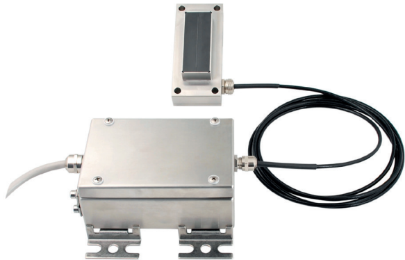
Transmitter in stainless steel housing with SONO- MIX Mini Standard probe
